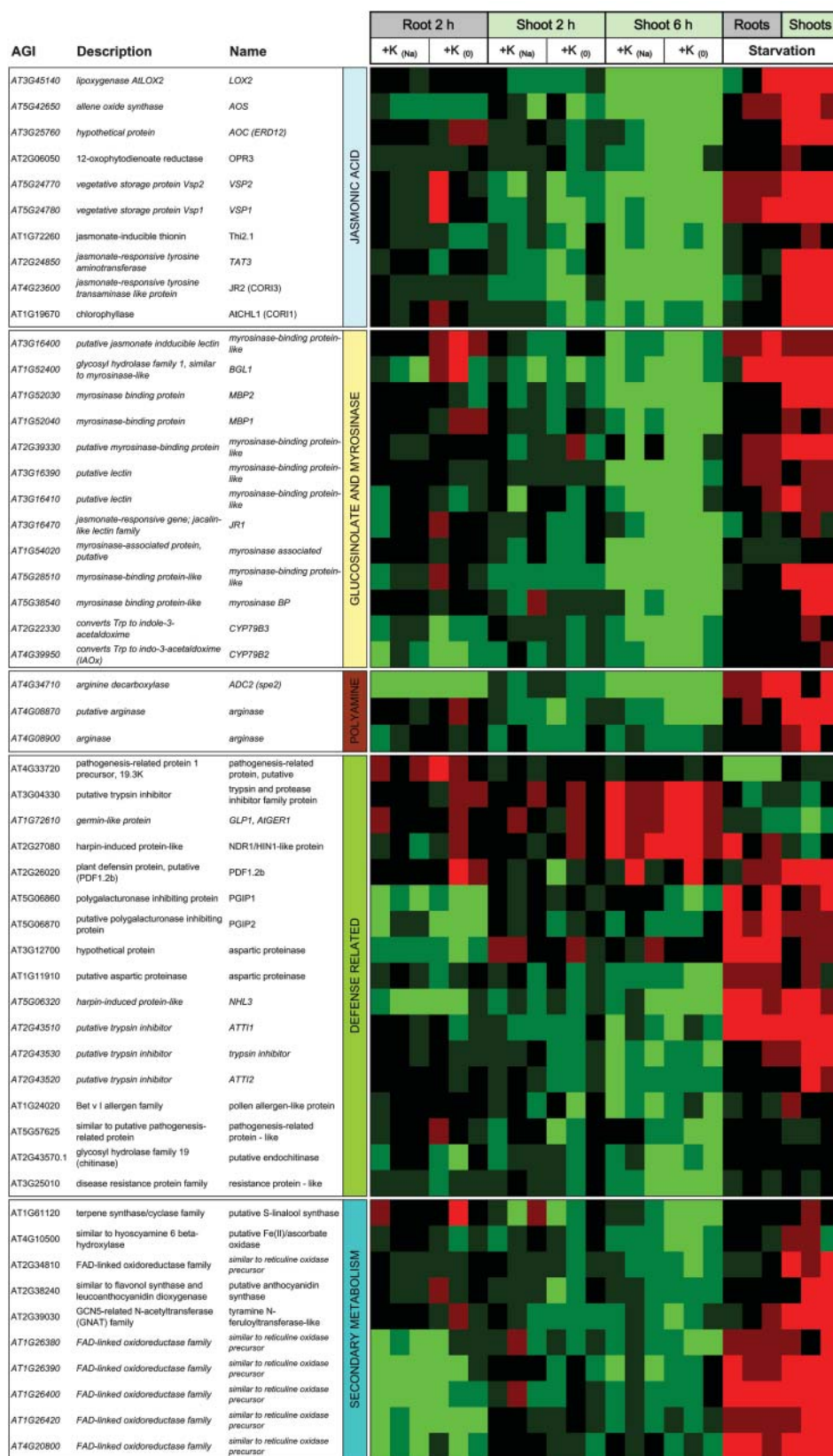
Figure 3. Expression profiles of highly significant K + -responsive genes related to JA-related genes were extracted from RP lists by FDR below 0.001%. On the left side AGI number, common name (if available) and a short description based on MIPS, TAIR, or TIGR are given for each gene. Genes identified by iGA are shown in italics. Functional super-categories extracted from iGA (Tables II–V) are given as vertical labels. On the right side expression profiles over all experimental conditions (compare Fig. 1C) are shown. Tissues and treatments are given on the top. Colors indicate change of transcript level in the treated samples with respect to the control samples (red for up-regulation, green for down-regulation, see color bar at the bottom of Fig. 4). For resupply treatments (+K + ) respective controls are given in brackets (Na for supply of Na + instead of K + , 0 for supply of K + -free medium). K + -starved plants were compared to plants grown on K + -sufficient medium. For each comparison data from three replicate experiments are shown.
